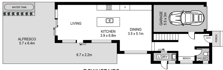
DOWNSTAIRS
