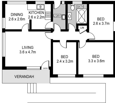
MAIN DWELLING
